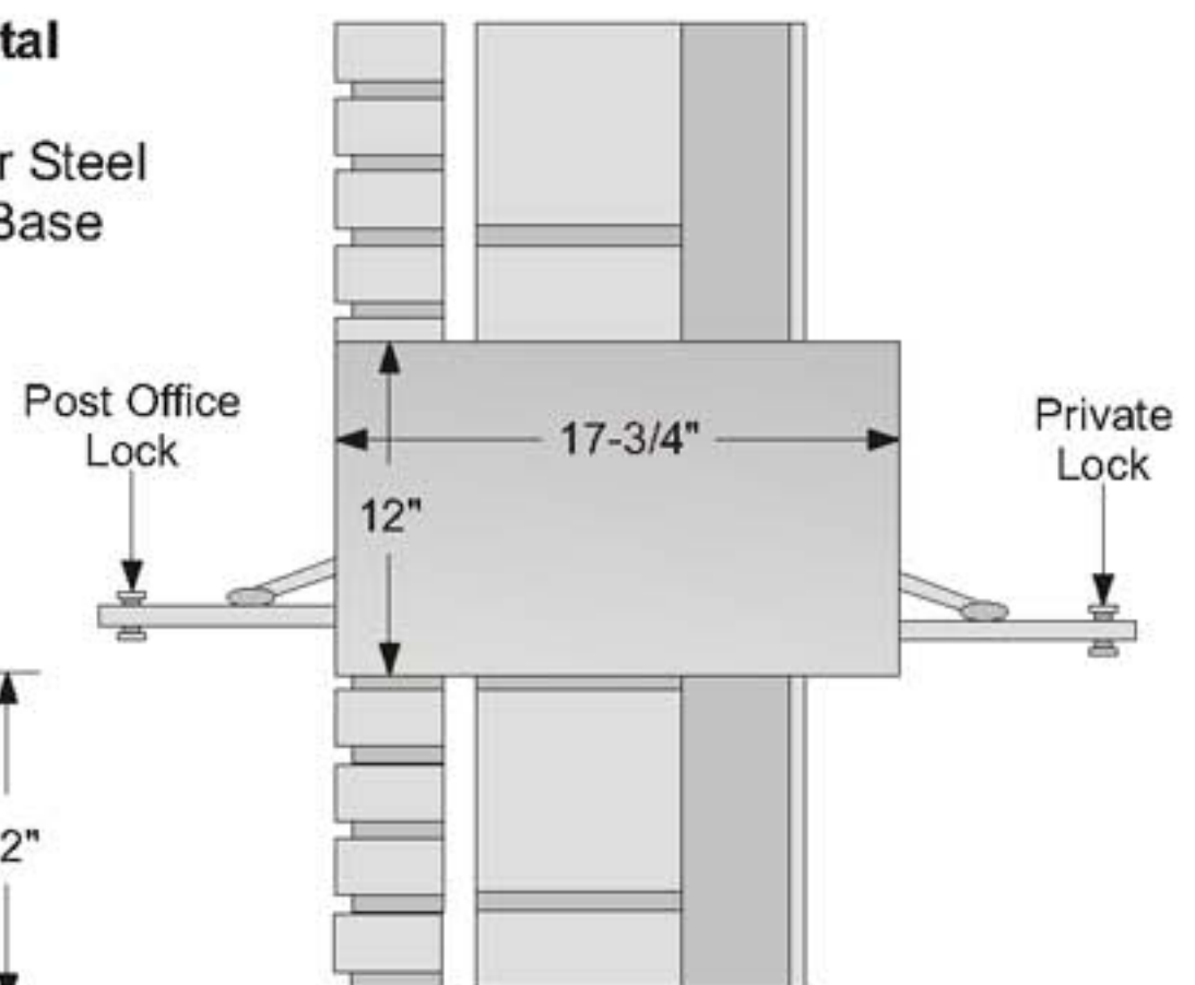
R924 Series - Through Wall
